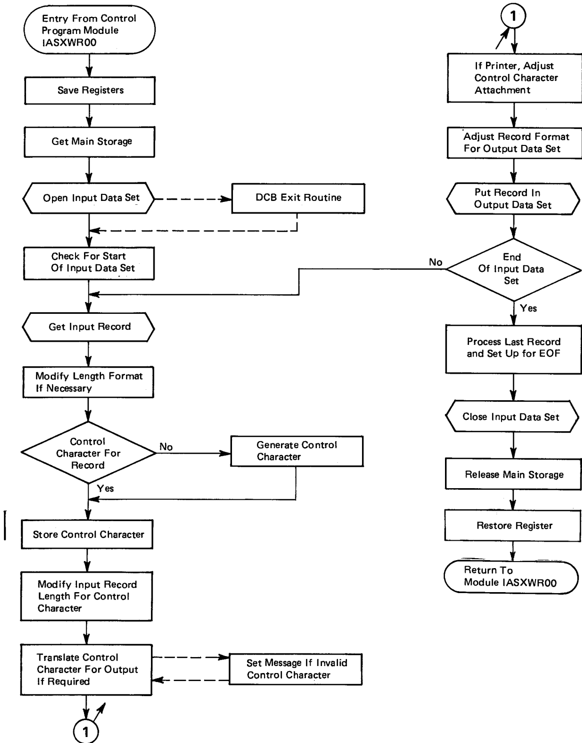
Figure 22. General Logic of Standard External Writer Routine
