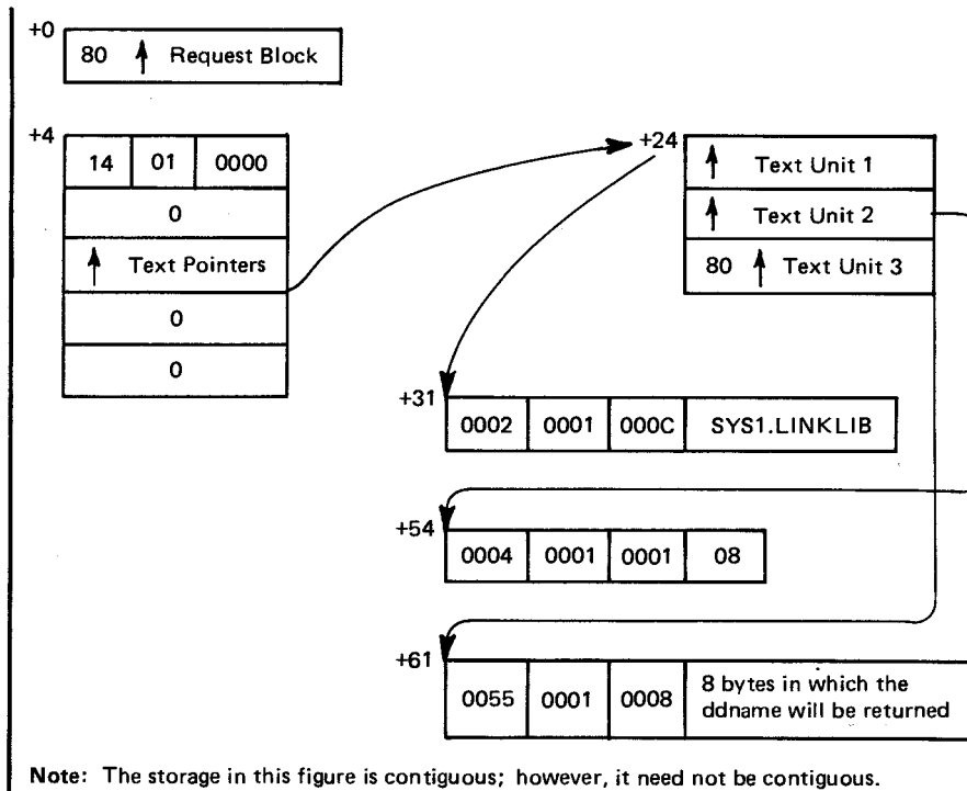
Figure 18. Resulting Parameter List From Dynamic Allocation Example
