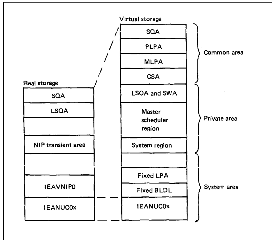
Figure 4.5. Initializing the Master Address Space
