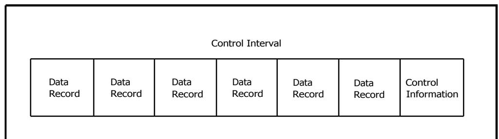
Figure 8.10. Data Records and Control Information Placement
