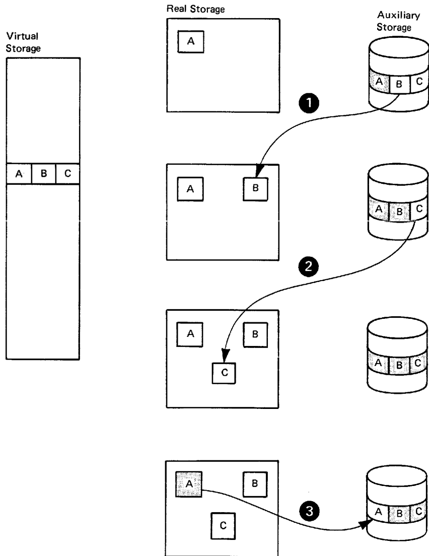
Figure 2.1. Basic Virtual Storage Concepts
