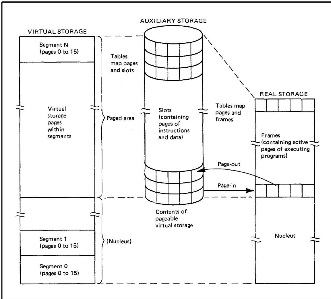
Figure 2.8. Page-out and Page-in
