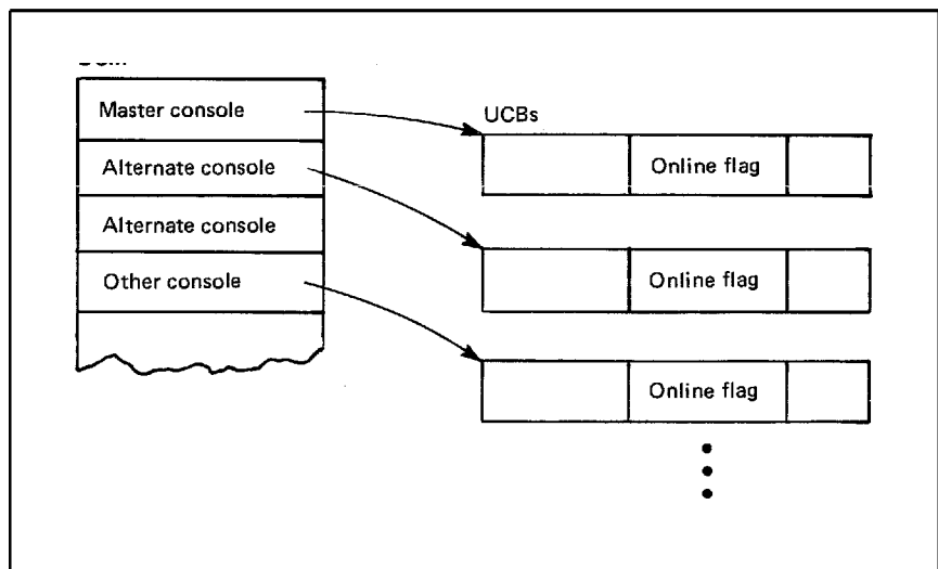
Figure 4.9. Locating a Master System Console
