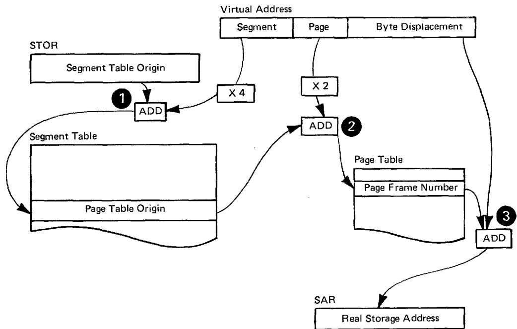
Figure 2.6. Dynamic Address Translation
