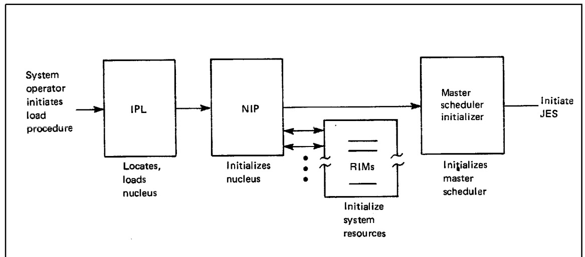
Figure 4.1. System Initialization Summary
